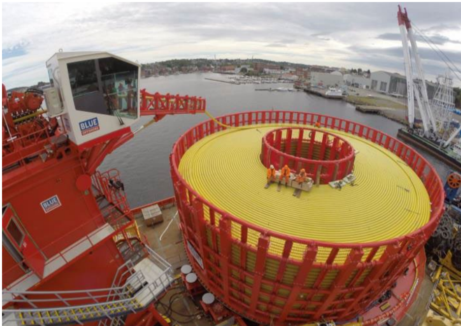
Figure 3 • Blue Offshore's BC01 loading ZOHR umbilical.
