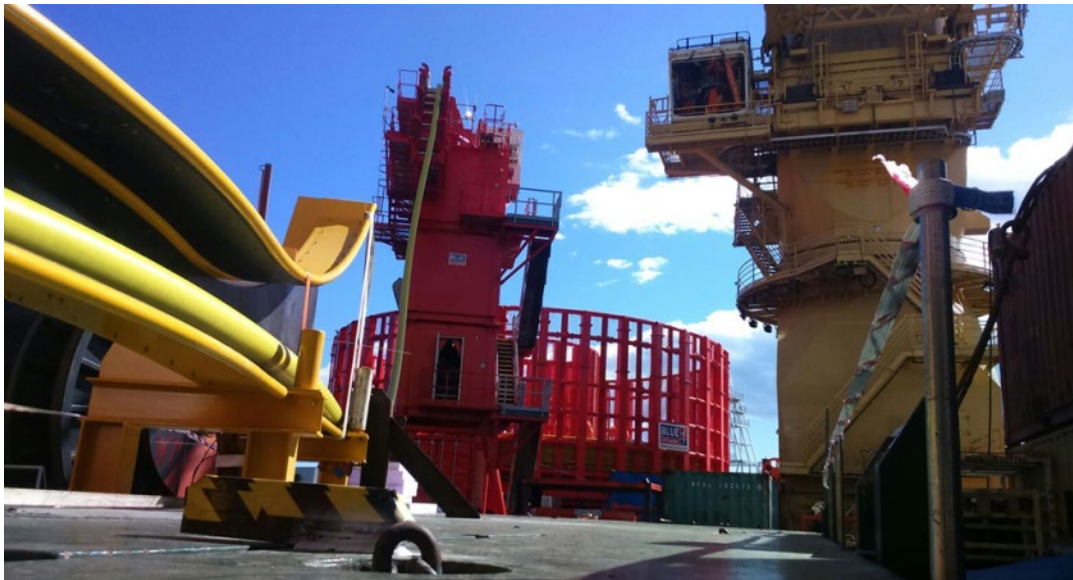
Figure 2 • Blue Offshore's BC01 on Normand Maximus loading ZOHR umbilical.
