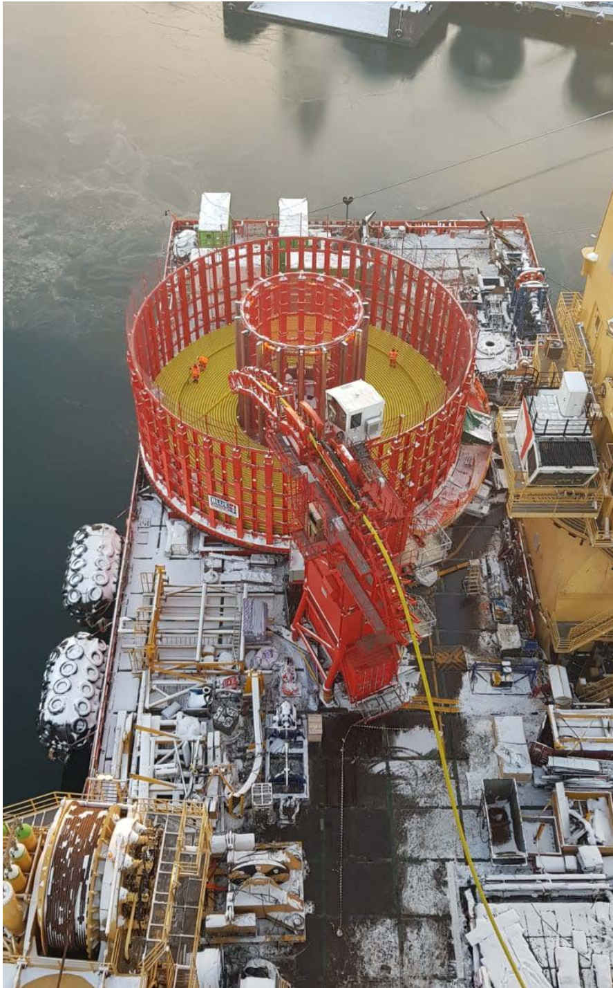
Figure 2 • Blue Offshore's BC01 on Normand Maximus umbilical transpooling operations at Aker, Norway.
